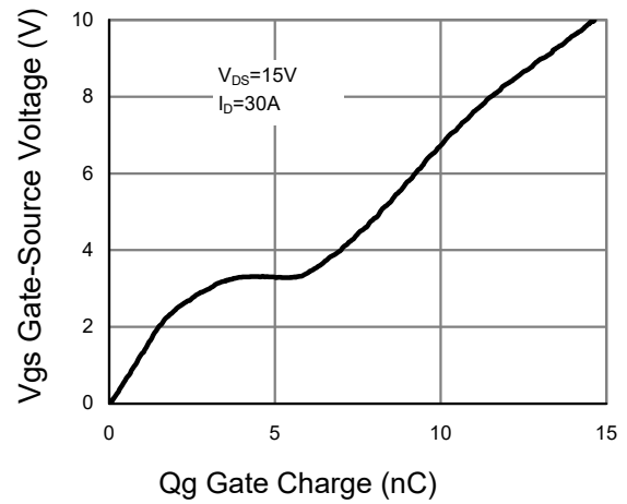
Fig. 5 Gate Charge
