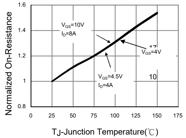
Fig. 4 Rds(on)-Junction Temperature
