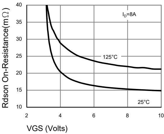
Fig. 3 On-Resistance vs. Gate-Source Voltage (Note E)
