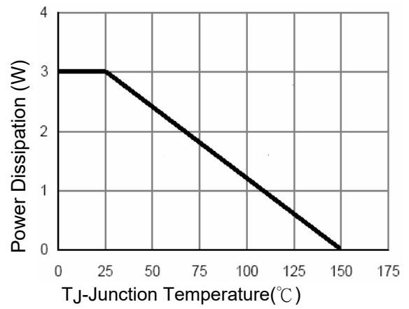
Fig. 8 Power De-rating
