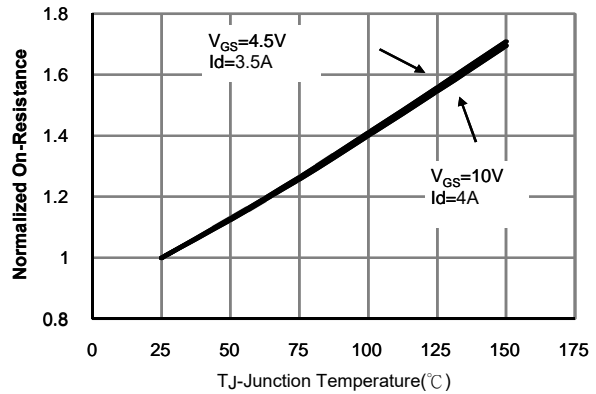
Fig. 4 Drain-Source On-Resistance (Note E)
